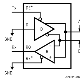
FIGURE 5. The DS36277 in a SAE J1708 Application
