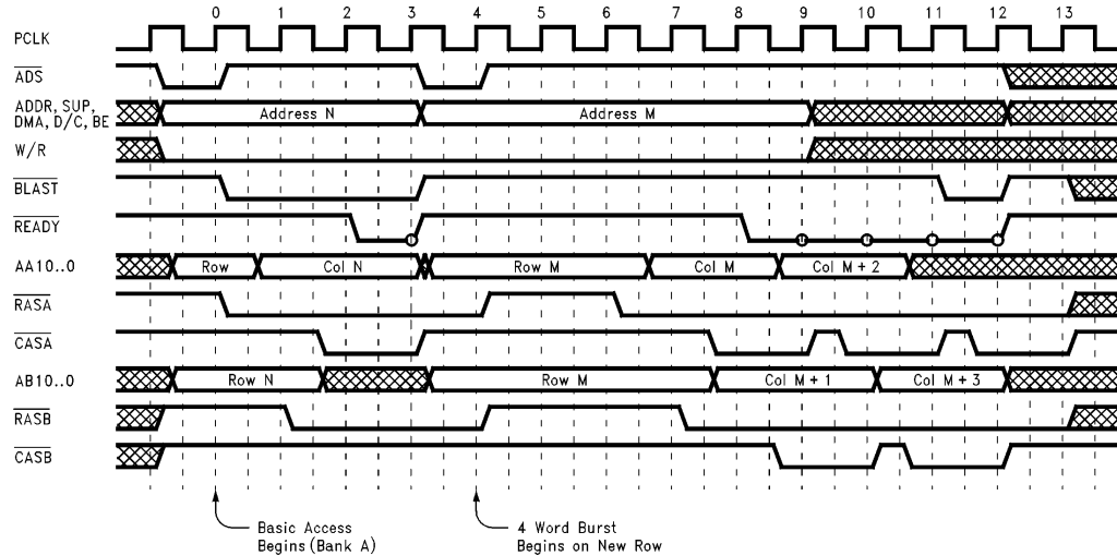
FIGURE 2.3.3. NSBMC096 with Row Compare Enabled: Row "Miss"
