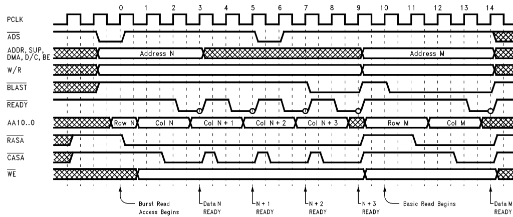
FIGURE 2.4. Non-Interleave Read/Write Access
