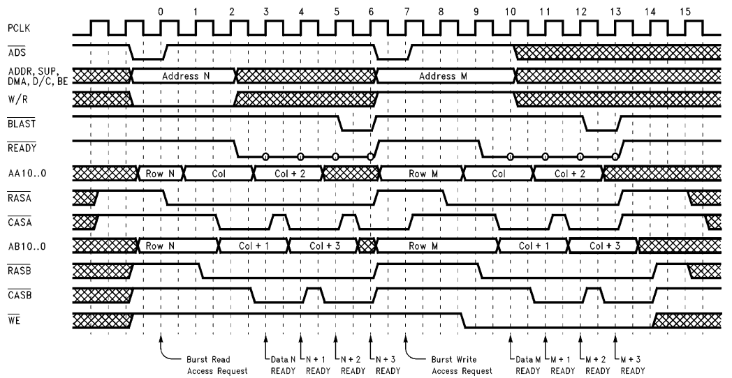
FIGURE 2.2.1. Burst Read Followed by Burst Write Access
