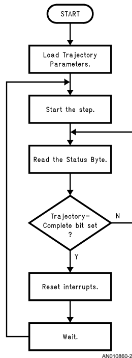
FIGURE 19. Step Generation Section of Filter Tuning Program
