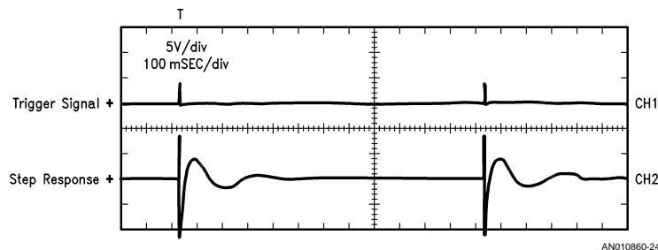
FIGURE 21. The Step Response of an Under Damped Control System
