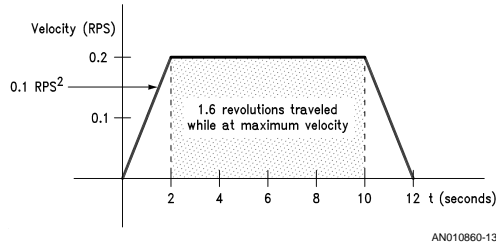
FIGURE 10. Velocity Profile for Simple Absolute Position Move Program
