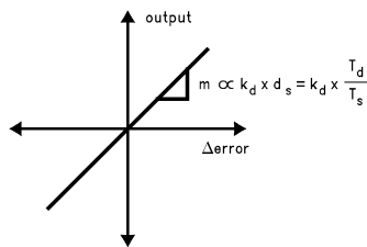
FIGURE 18. Proportional, Integral, and Derivative (PID) Force Components
