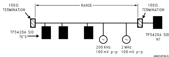
FIGURE 3. SID Point-to-Point Range Measurement
