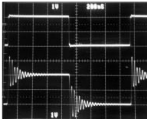
FIGURE 11A. Pulse Response of LH4101 Driving a 220 pF Load with R_1 = 8\Omega
