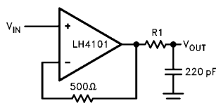
FIGURE 12. Compensation for Capacitive Load
