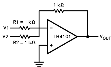
FIGURE 7. Summing Amplifier
