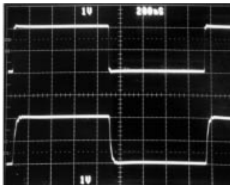
FIGURE 11B. With R_1 = 50\Omega
