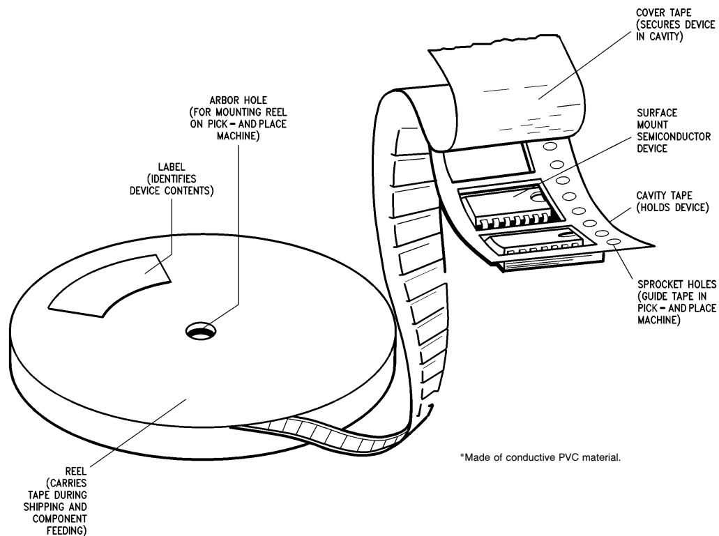
FIGURE 5. Tape-and-Reel Diagram
