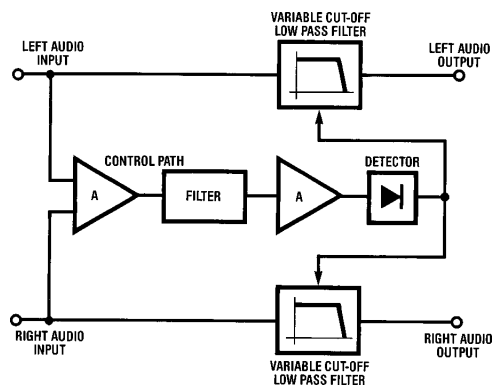
FIGURE 2. Stereo Noise Reduction System (DNR) TL/H/8389-2
