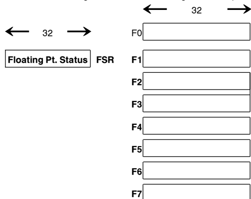
FIGURE 1. FPU Registers
