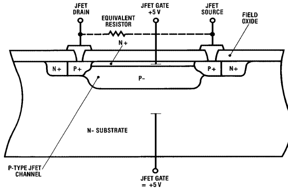
FIGURE 6. P-Pinched Resistor
