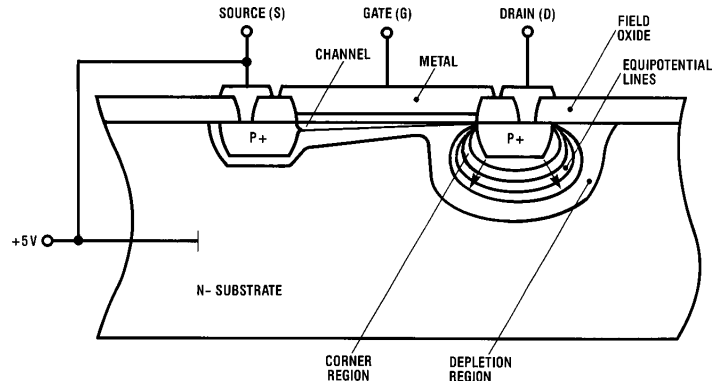
FIGURE 5. Surface Avalanche Breakdown in a CMOS P-Channel Transistor
