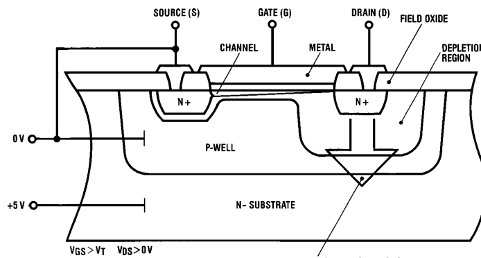
FIGURE 3. Vertical Punchthrough in a CMOS N-Channel Transistor
