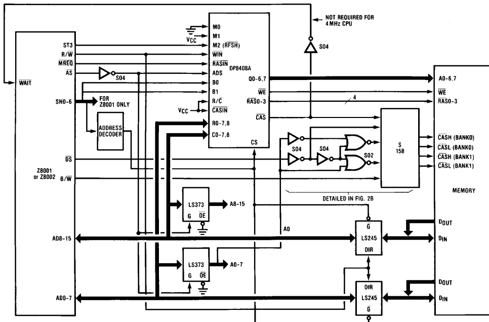
FIGURE 2a. Z8000 and DP8408A Interface
