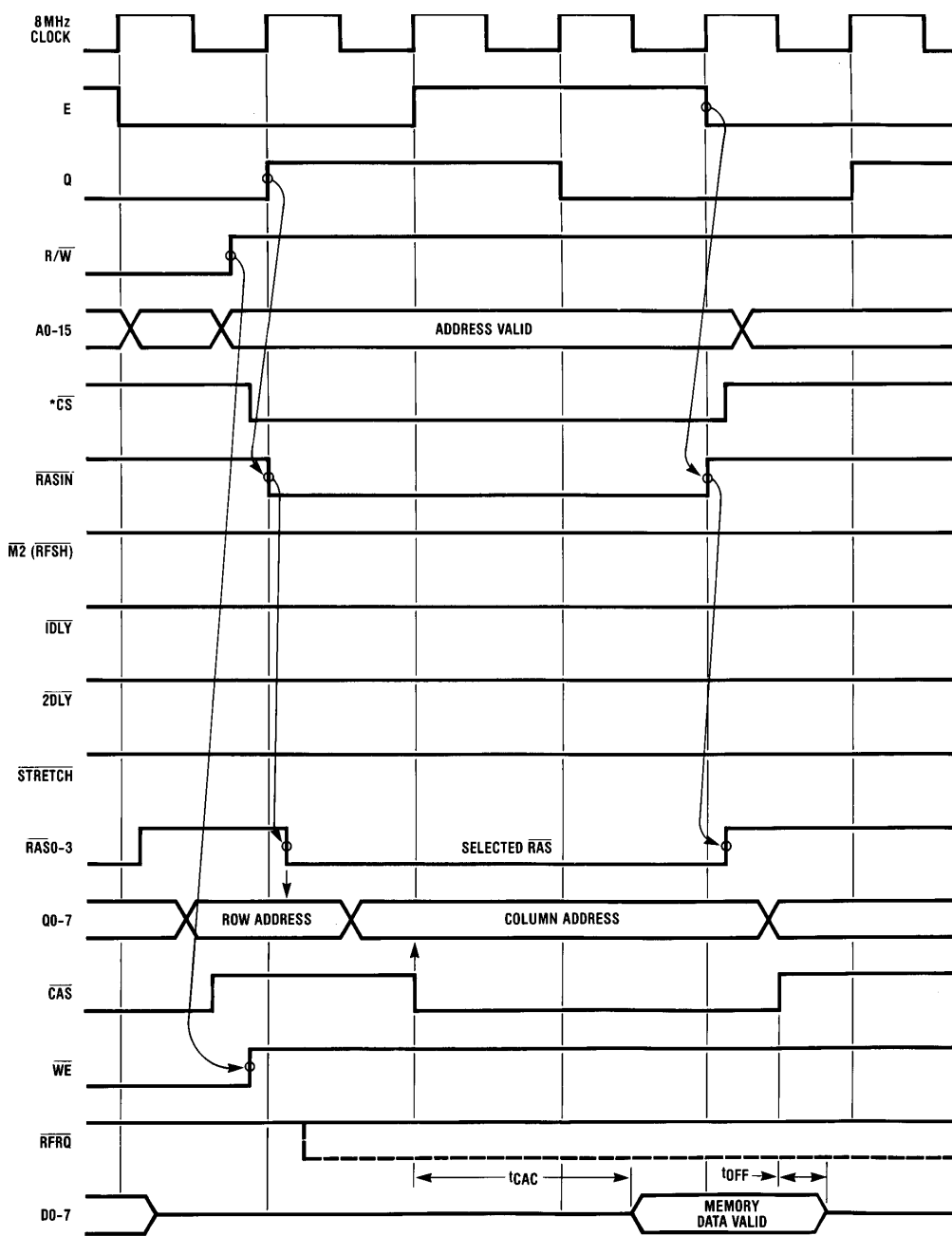
FIGURE 12. MC68B09E Memory Read Cycle
