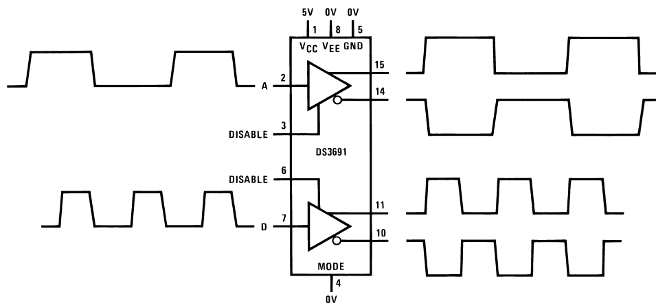
FIGURE 10. DS3691 Connected for Balanced Mode Operation
