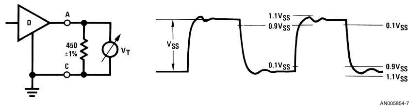
FIGURE 6. Unbalanced Driver Output Signal Waveform
