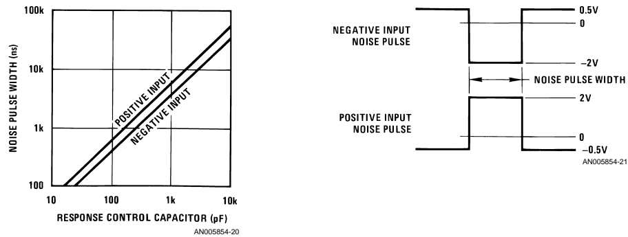
FIGURE 17. Noise Pulse Width vs Response Control Capacitor
