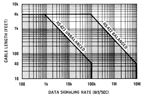
FIGURE 3. Data Signaling Rate vs Cable Length
