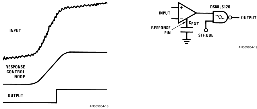
FIGURE 16. Application of DS88LS120 Receiver Response Control and Hysteresis
