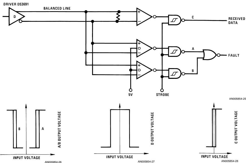
FIGURE 19. Fail-Safe Using the DS88LS120 Threshold Offset for Balanced Lines
