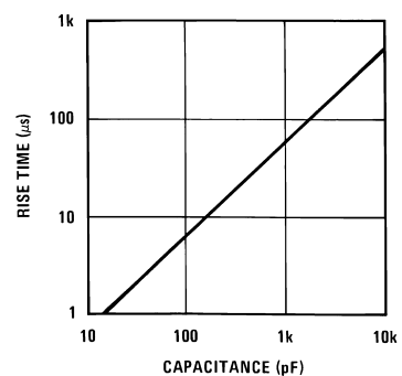
FIGURE 13. DS3691 Rise Time vs External Capacitor
