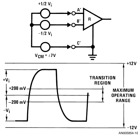
FIGURE 8. Receiver Input Sensitivity Measurement
