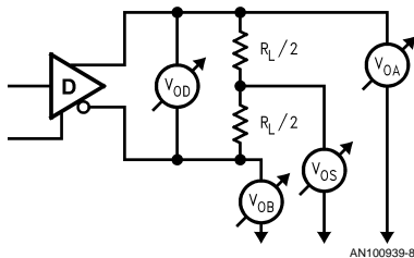
FIGURE 6. V_{OA} , V_{OB} , V_{OD} , and V_{OS} Driver Measurements
