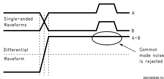
FIGURE 8. Coupled Noise is Common Mode and is Rejected
