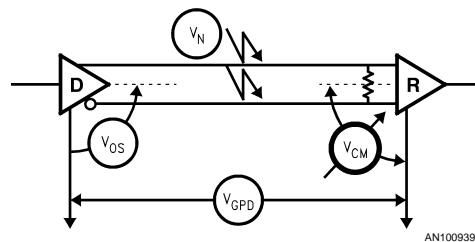
FIGURE 7. The Three Components of V_{CM}
