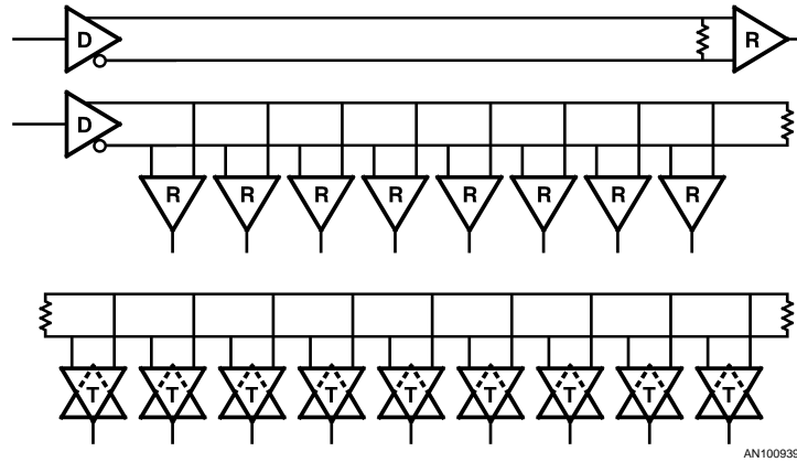
FIGURE 3. Bus Configurations: Point-to-Point, Multi-Drop, and Multi-Point
