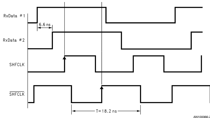
FIGURE 2. Data Correctly Reconstructed at 55 MHz
