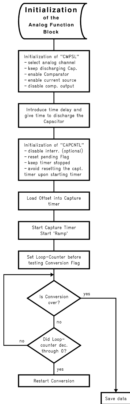
FIGURE 4. "Flowchart" A/D Conversion Initialization
