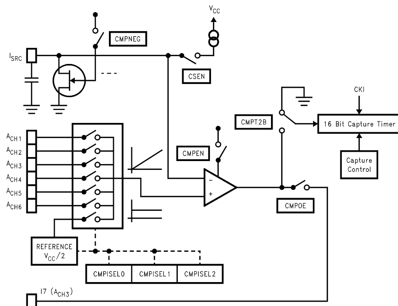
FIGURE 2. Analog Function Block and Control Bits
