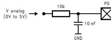
FIGURE 38. Example of Analog Input Components
