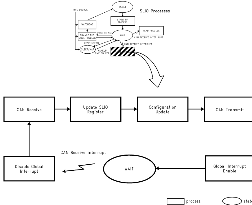
FIGURE 12. Update Process
