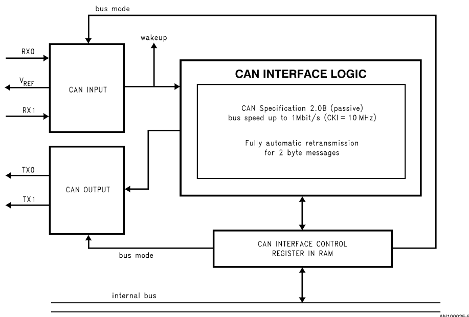
FIGURE 5. CAN Interface Block Diagram
