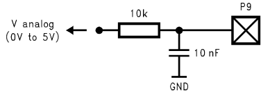
FIGURE 40. Example of Analog Output Components
