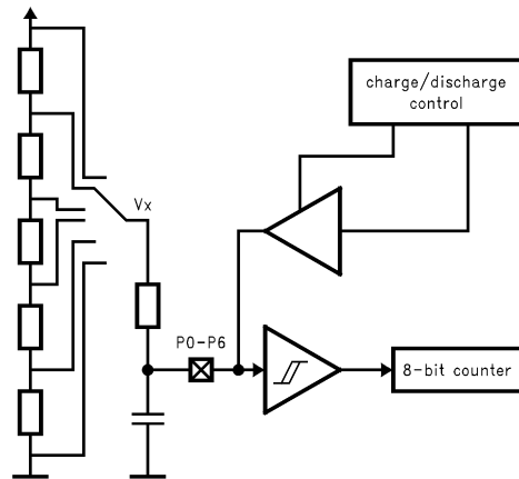
FIGURE 13. Analog Input
