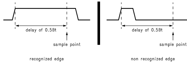
FIGURE 42. Delay Time External Rising Event
