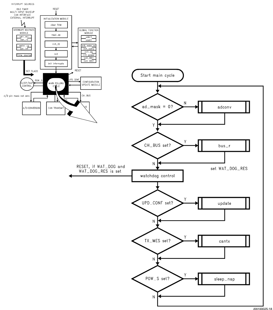
FIGURE 18. Flow of Main Polling Cycle
