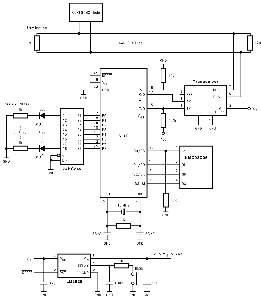
FIGURE 45. SLIO Node Schematic
