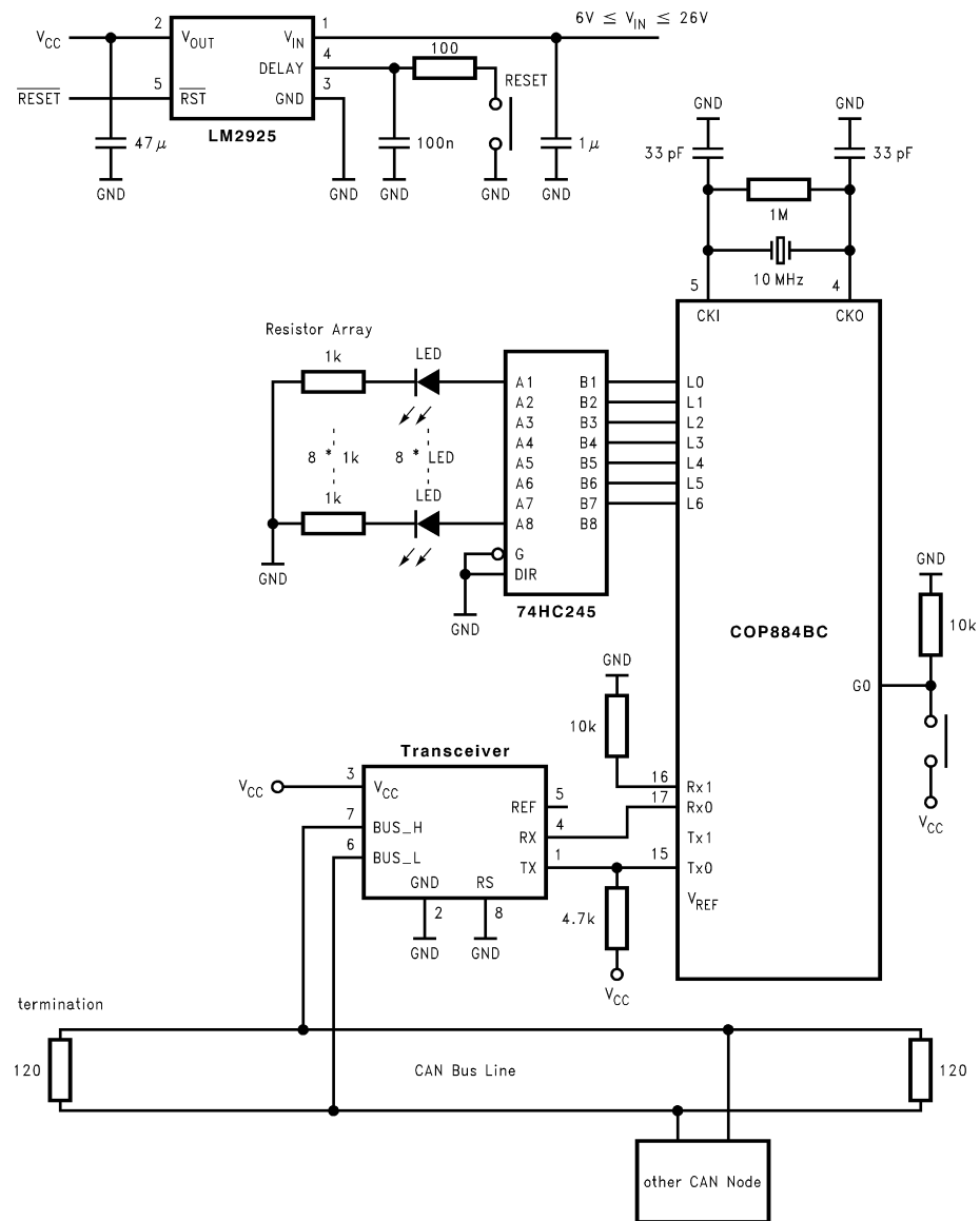
FIGURE 44. COP884BC Node
