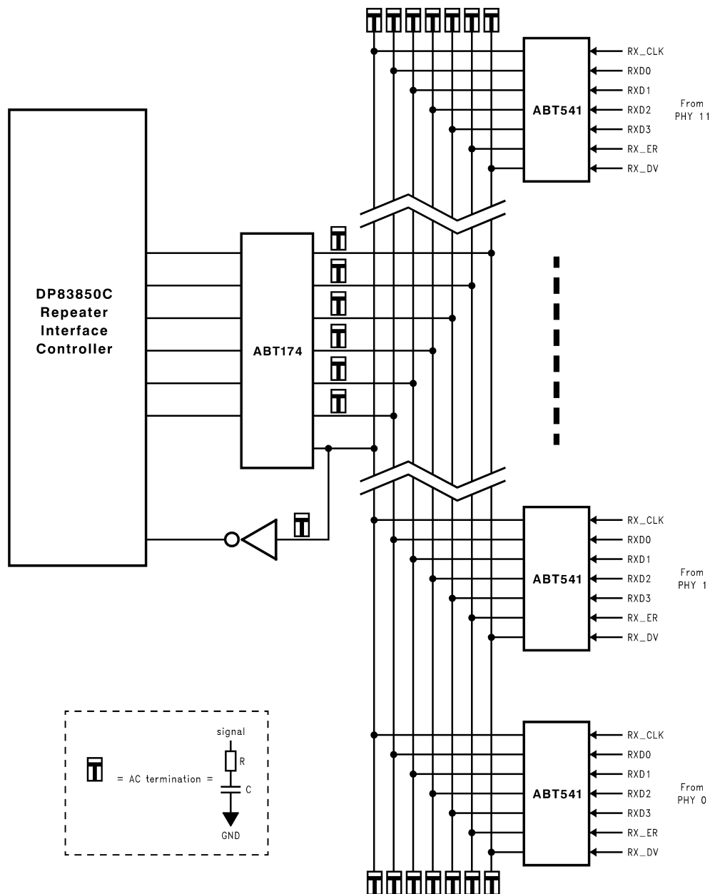
FIGURE 11. MII Receive BUS Termination
