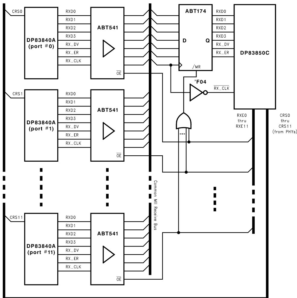
FIGURE 10. MII Receive Interconnection Recommendation
