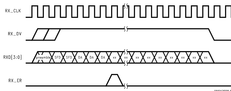
FIGURE 8. MII Reception with Error(s)
