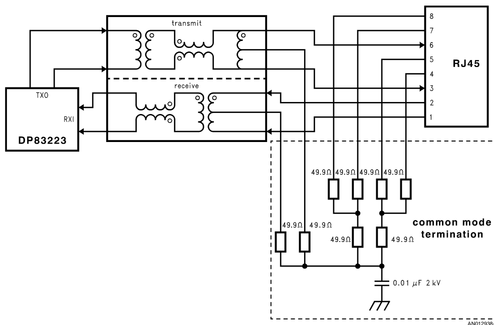
FIGURE 3. PMD Magnetics
