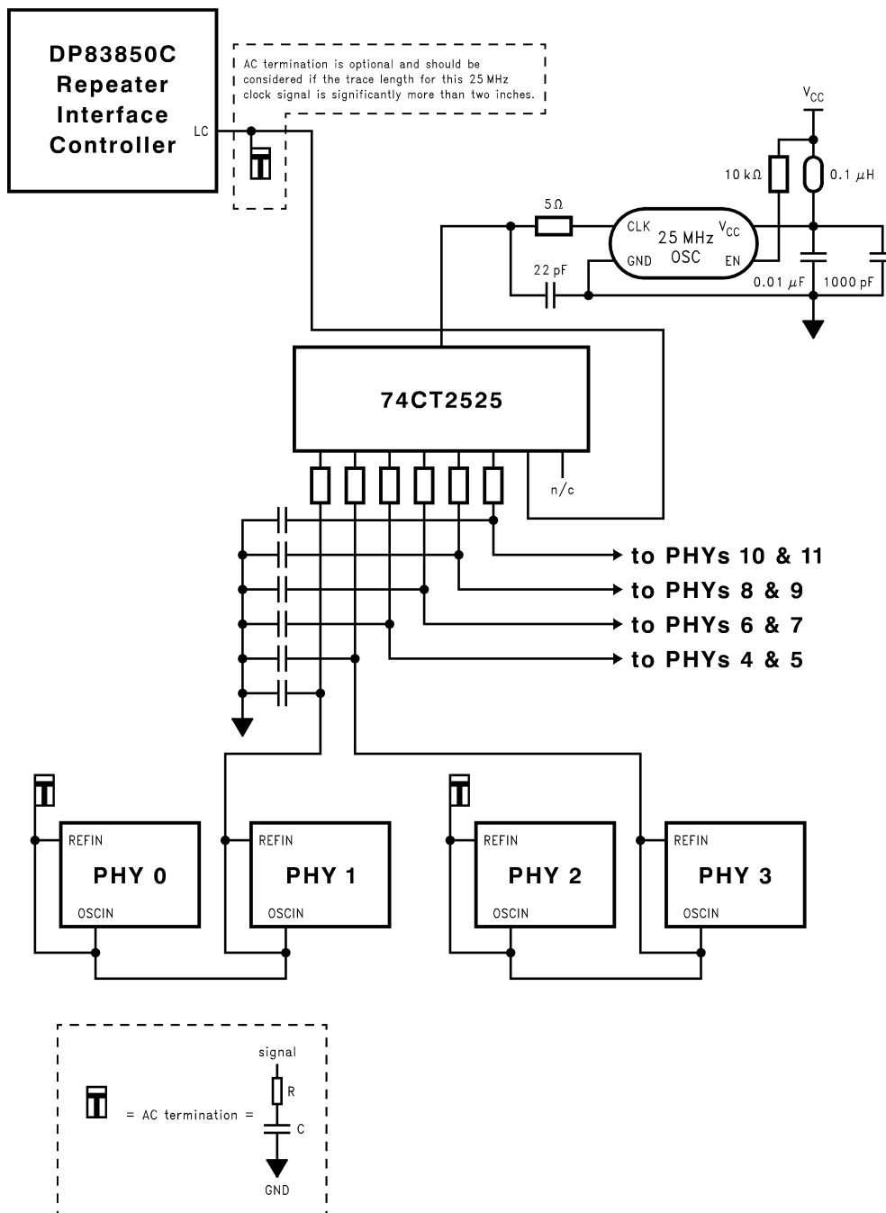
FIGURE 17. Reference Clock Recommendation for Non-Auto-Negotiating 100BASE-TX Repeater
