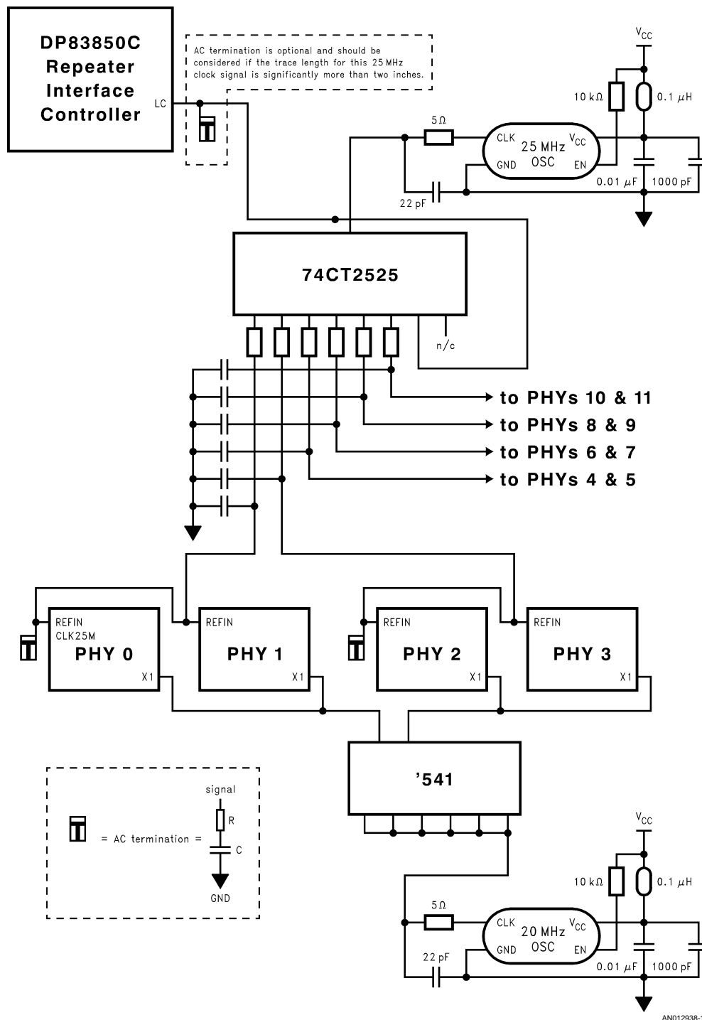
FIGURE 18. Reference Clock Recommendation for Auto-Negotiating 100BASE-TX Repeater
