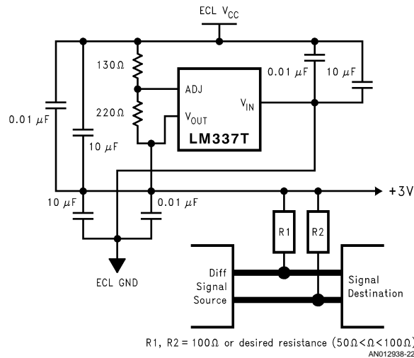
FIGURE 22. Direct PECL Termination
