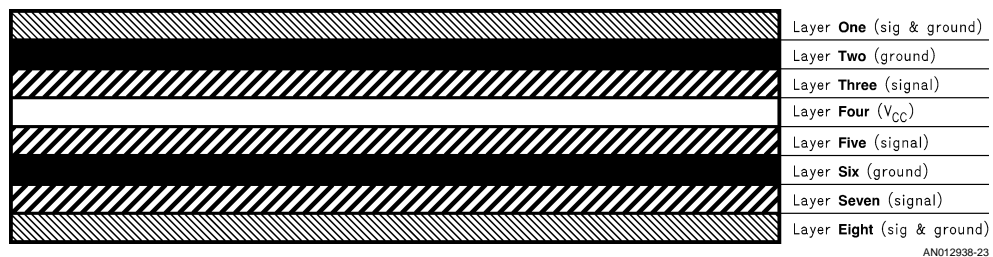
FIGURE 23. Typical Board Layer Assignment
