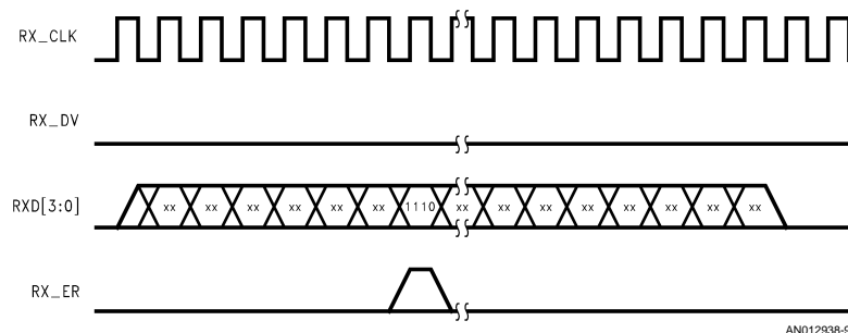
FIGURE 9. False Carrier Indication
