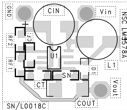
FIGURE 6. PCB Layout for the Circuits Shown in Figures 3, 4 (Scale: 2:1)
