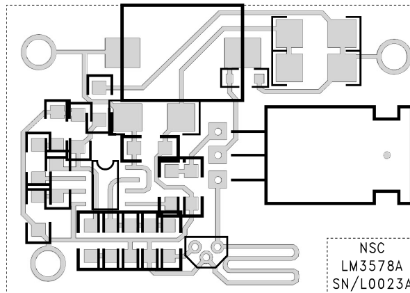
FIGURE 7. PCB Layout for the Circuit Shown in Figure 5 (Scale: 2:1)
