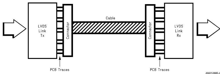
FIGURE 4. Interconnect Skew = PCB + Connector + Cable + Connector + PCB
