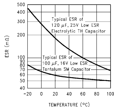
FIGURE 4. Capacitor ESR Changes vs Temperature
