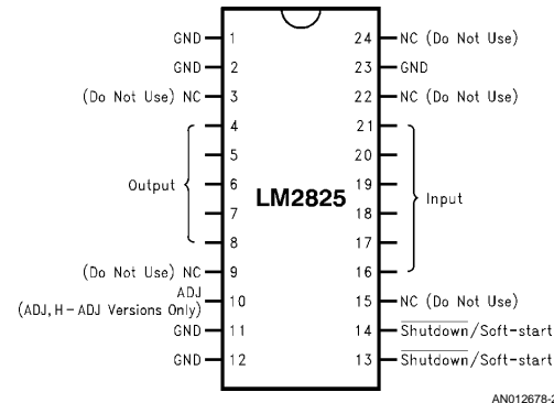
FIGURE 1. Connection Diagram
