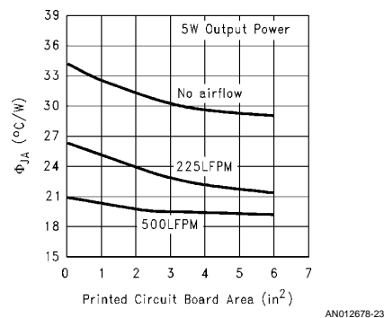
FIGURE 21. \theta_{JA} vs Board Area for 3 Windspeed Levels
