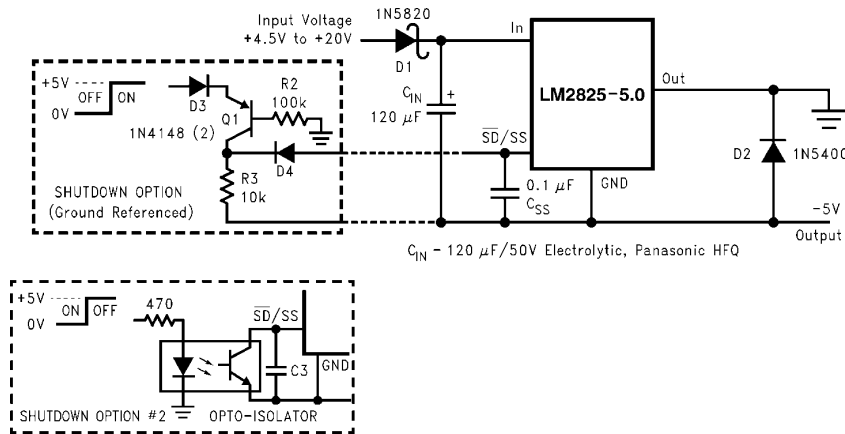
FIGURE 16. Inverting Regulator
