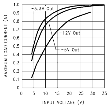
FIGURE 17. Inverting Regulator Typical Load Current
