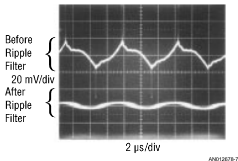
FIGURE 6. Post Ripple Filter Waveform
