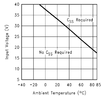
FIGURE 8. Usage of The Soft-Start Capacitor
