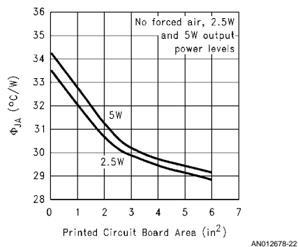
FIGURE 20. \theta_{JA} vs Board Area for 2 Output Power Levels
