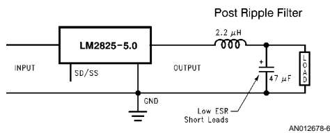
FIGURE 5. Post Ripple Filter
