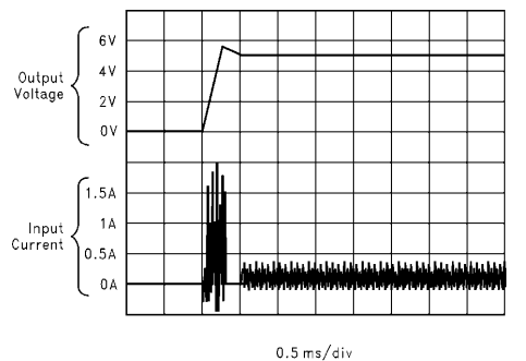
FIGURE 7. Output Voltage and Input Current during Start-Up
