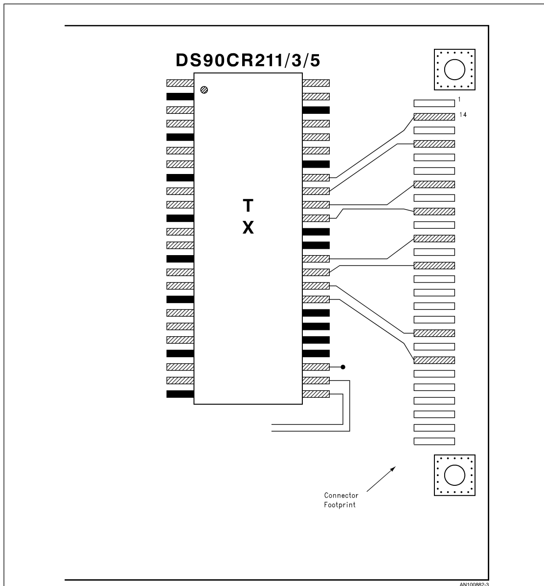
FIGURE 3. LVDS PCB Layout
