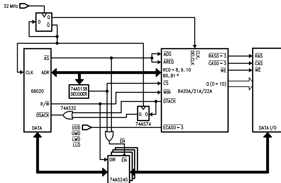
FIGURE 1. Design # 1, 68020 up to 16 MHz with 1 Wait State
