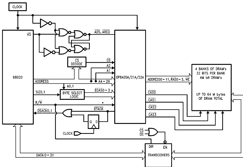
FIGURE 4. 68020 Design #2
