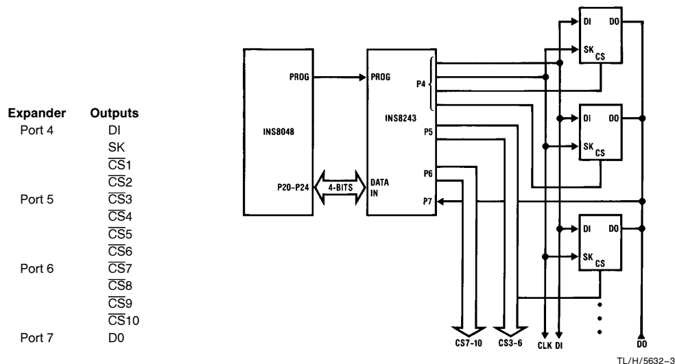
FIGURE 5. I/O Expansion
