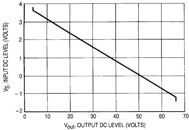
Figure 1. V_S versus V_{out}
