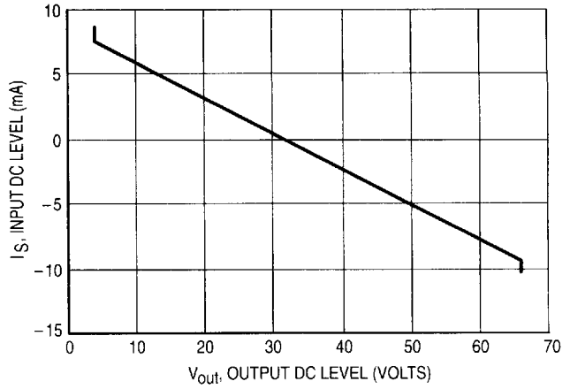
Figure 2. I_S versus V_{out}
