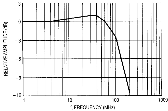
Figure 3. Frequency Response
