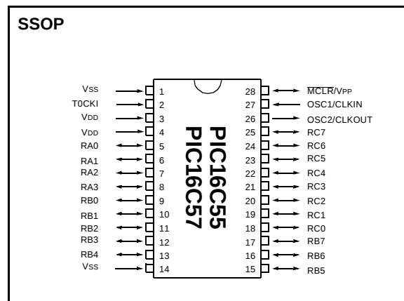
FIGURE 0-1: CORRECTED SSOP PIN-OUT
