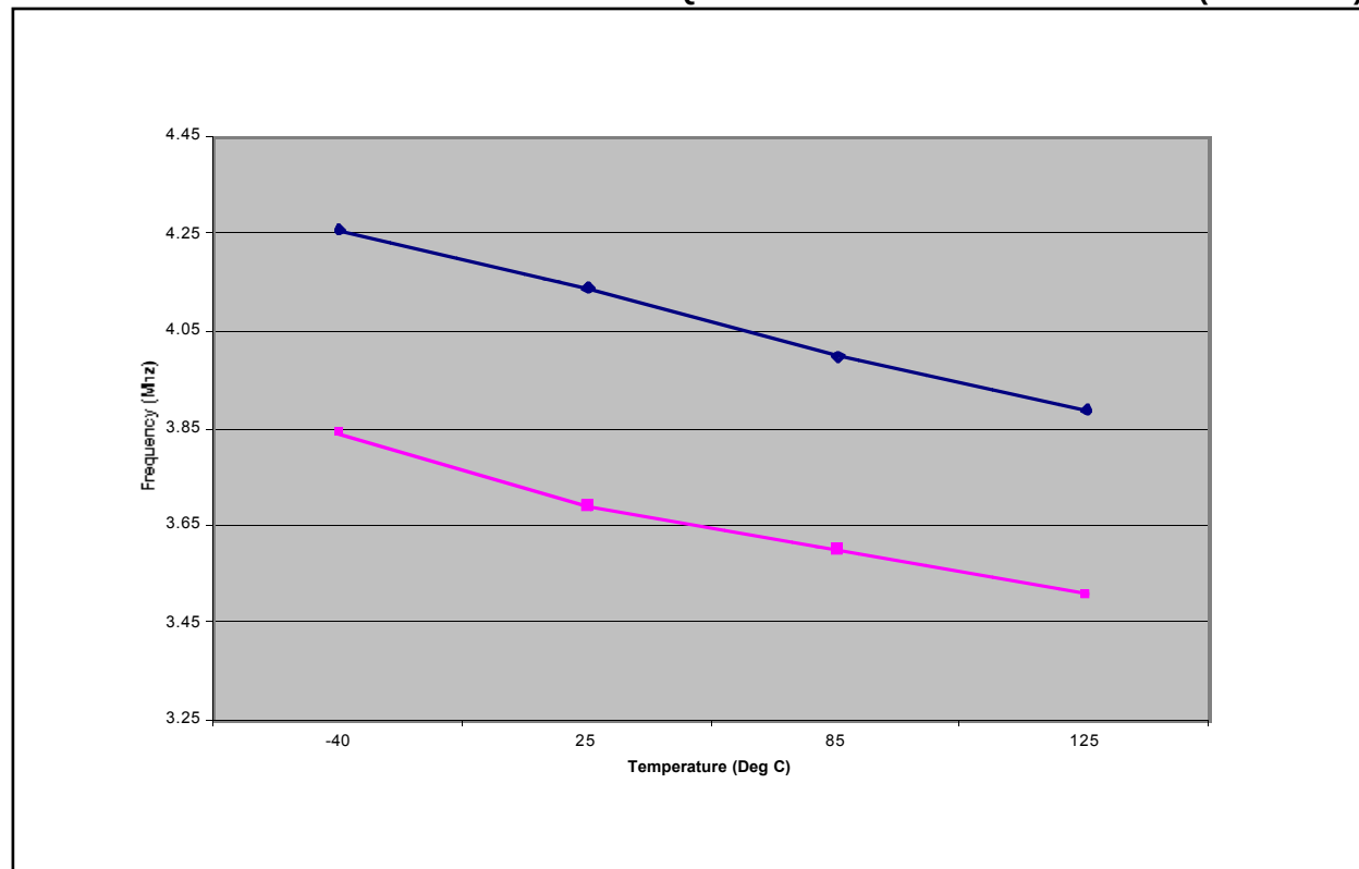
FIGURE 11-1: CALIBRATED INTERNAL RC FREQUENCY RANGE VS. TEMPERATURE ( V_{DD} = 2.5V )
