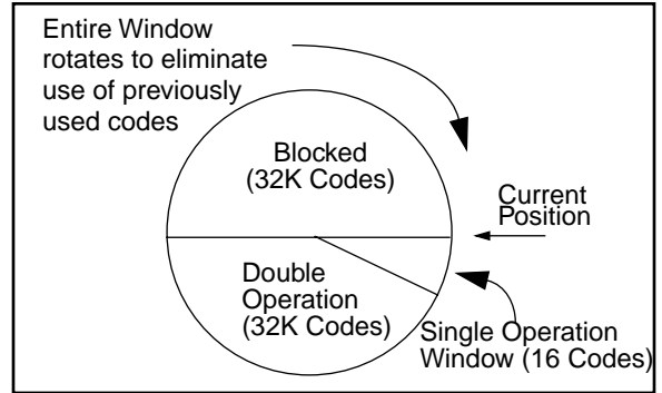
FIGURE 4-5: SYNCHRONIZATION WINDOW
