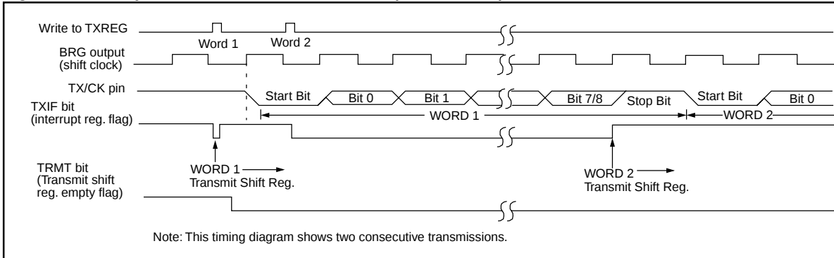
Figure 18-3: Asynchronous Master Transmission (Back to Back)
