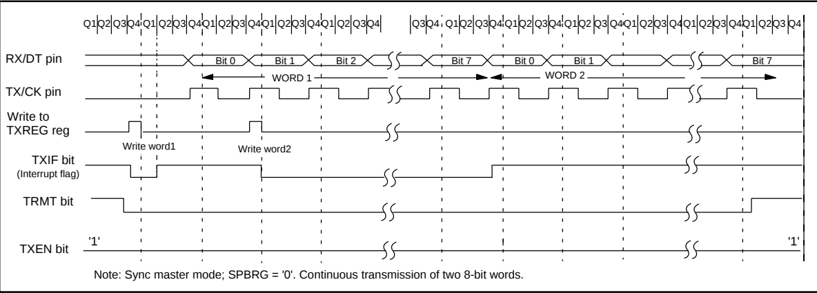
Figure 18-10: Synchronous Transmission
