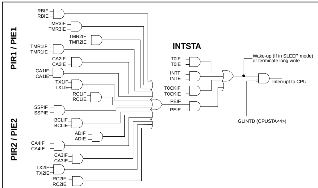
FIGURE 6-1: INTERRUPT LOGIC
