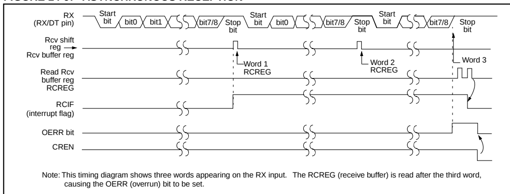
FIGURE 14-9: ASYNCHRONOUS RECEPTION
