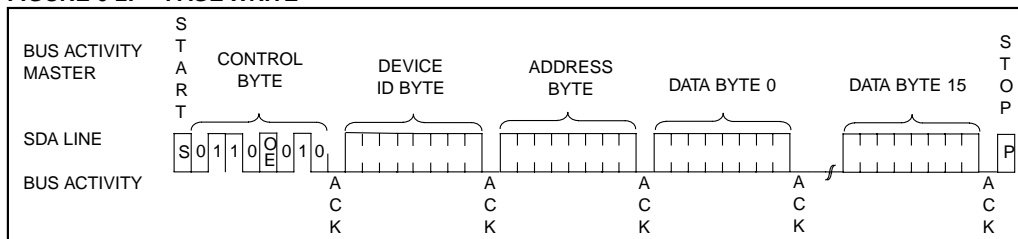
FIGURE 6-2: PAGE WRITE
