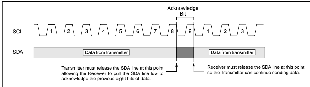
FIGURE 3-2: ACKNOWLEDGE TIMING
