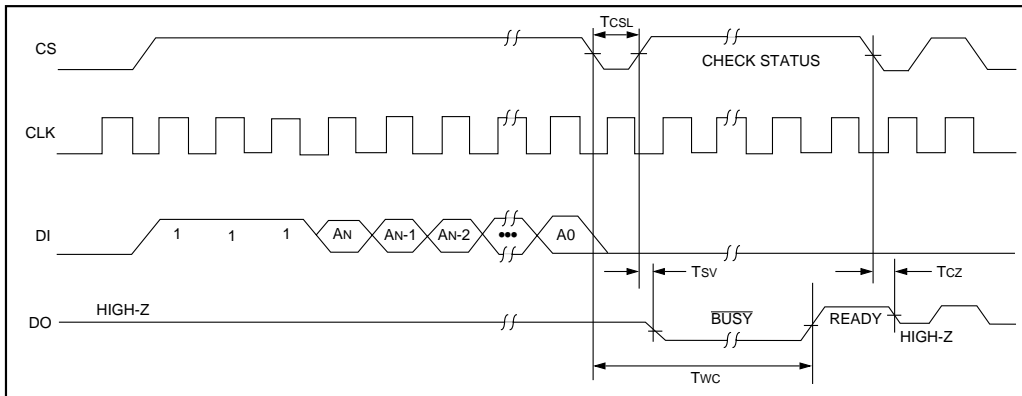
FIGURE 3-2: ERASE TIMING
