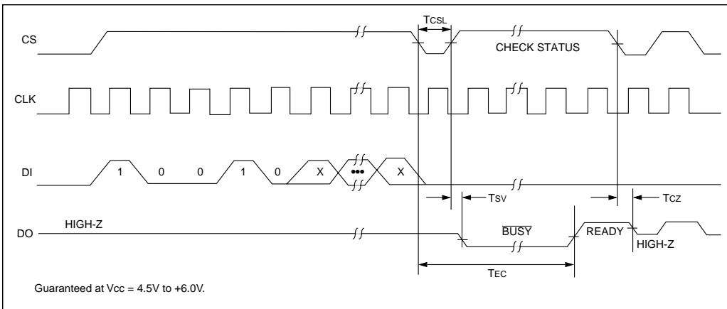
FIGURE 3-3: ERAL TIMING
