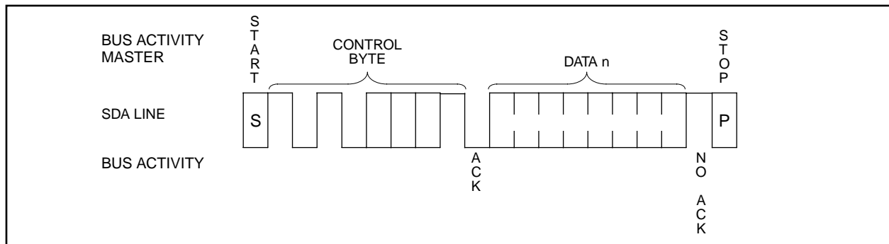
FIGURE 6-2: RANDOM READ
