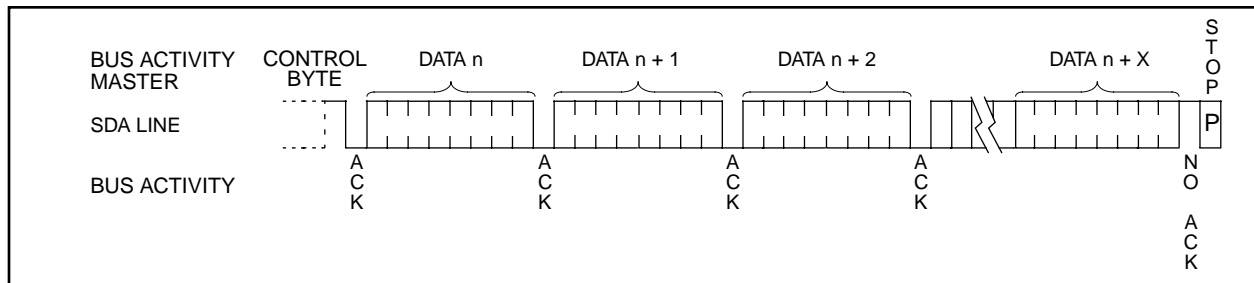
FIGURE 6-3: SEQUENTIAL READ
