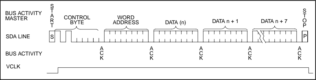
FIGURE 4-3: PAGE WRITE
