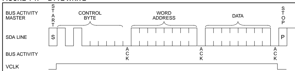
FIGURE 4-1: BYTE WRITE
