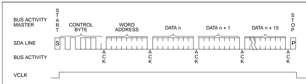
FIGURE 4-2: PAGE WRITE
