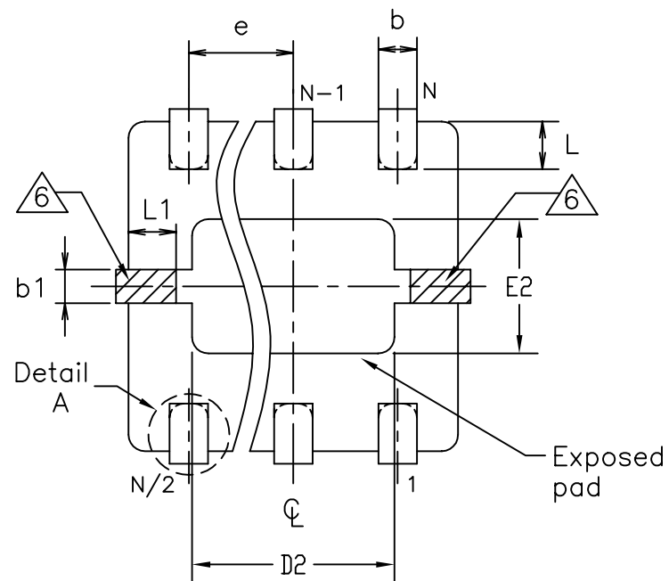
BOTTOM VIEW
