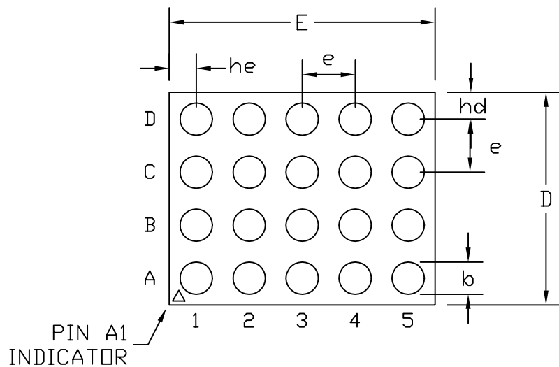
BOTTOM VIEW
