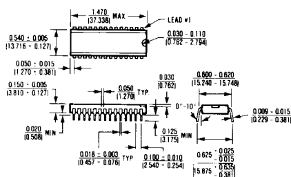
28 Lead Plastic DIP (PI)
