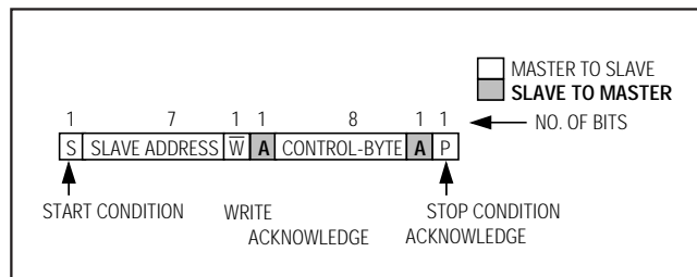
Figure 6. Write Cycle
