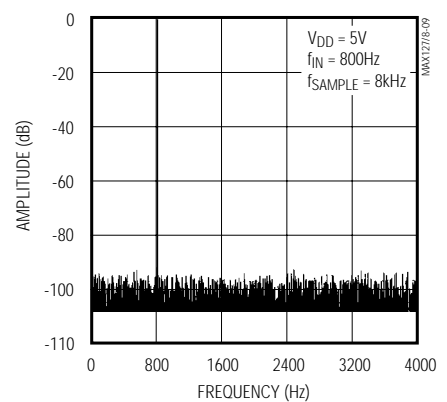
FFT PLOT
