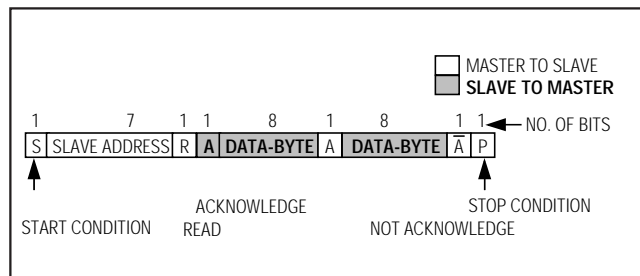
Figure 7. Read Cycle
