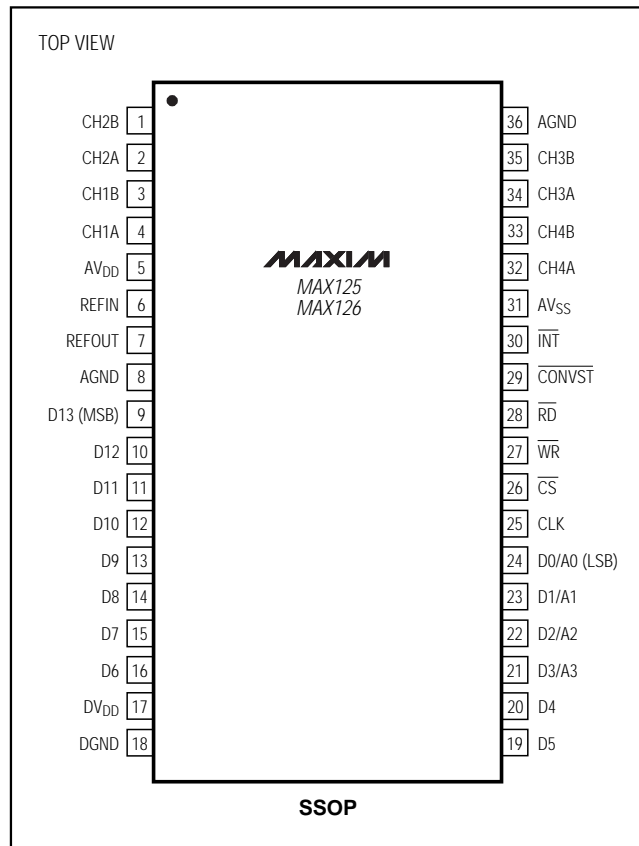
Pin Configuration
