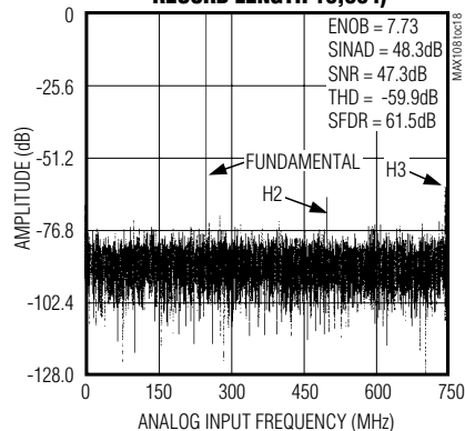
FFT PLOT ( f_{IN} = 1503.021240MHz , -3dBFS, RECORD LENGTH 16,384)
