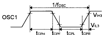
EXTERNAL CLOCK
