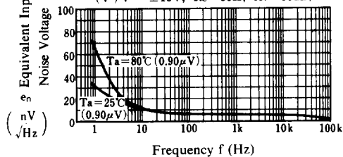
Equivalent Input Noise Voltage vs. Frequency
