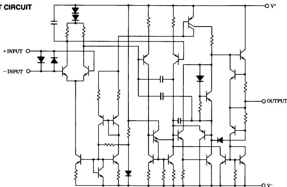
NJM5532D NJM5532M
