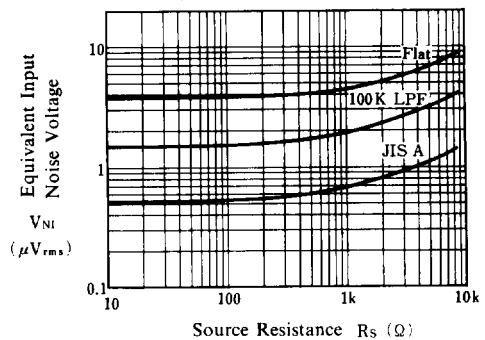
Equivalent Input Noise Voltage vs. R_s
