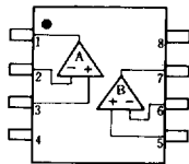
NJM4558D, NJM4558M, NJM4558V NJM4558D, NJM4558M, NJM4558V
