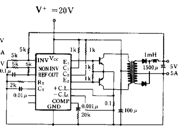
Fig. 3 Push-Pull Transformer-Coupled Circuit
