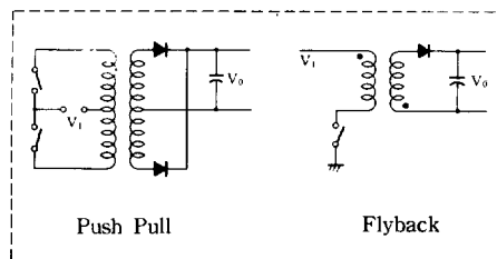
Transformer-Coupled Outputs
