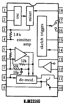
NJM3359D
