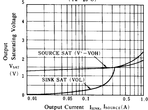
Output Saturating Voltage vs. Output Current
