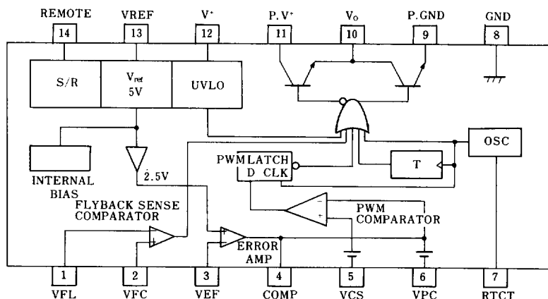
NJM2362D
