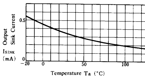
Output Sink Current vs. Temperature
