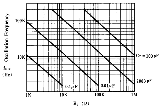
Oscillation Frequency vs. R_t , C_t
