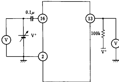
Test Circuit 3
