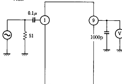
Test Circuit 10
