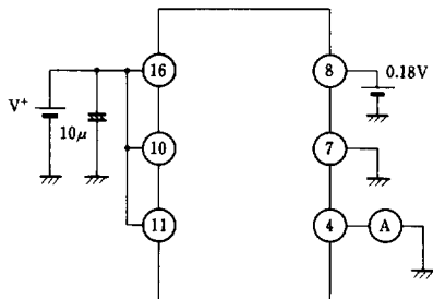
Test Circuit 13
