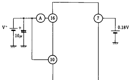
Test Circuit 13
