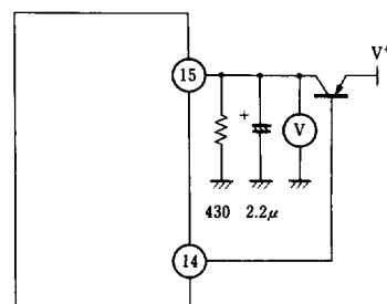
Test Circuit 8
