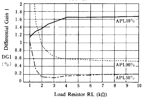
Differential Gain 1 vs. Load Resistor
