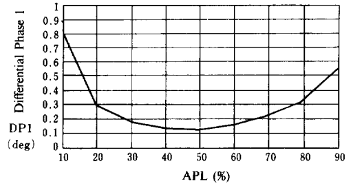
Differential Phase 1 vs. APL
