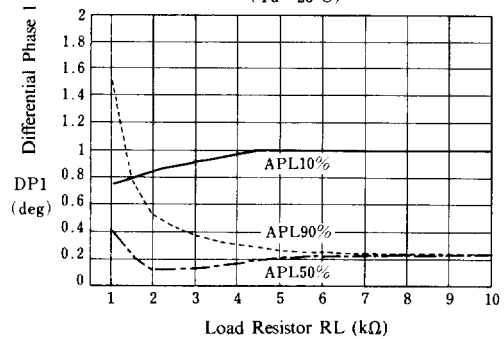
Differential Phase 1 vs. Load Resistor
