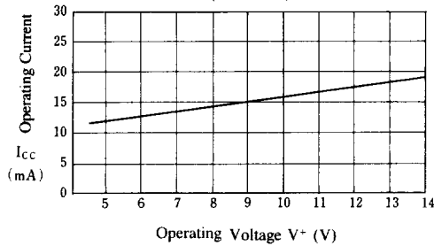
Operating Current vs. Operating Voltage
