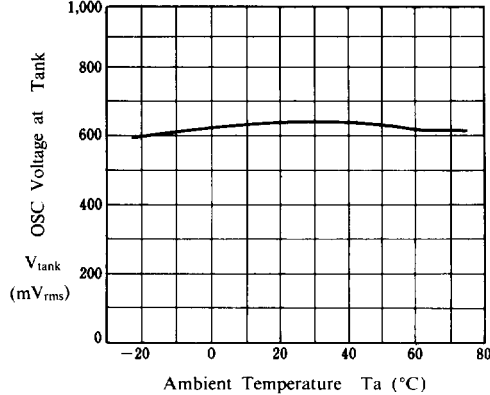
V_{\text{tank}} vs. T_a
