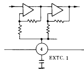
<Decoupling Capacitor>
